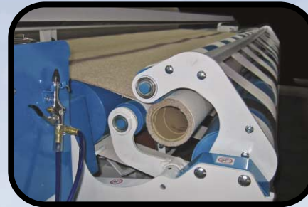
REVERSE ROLL
